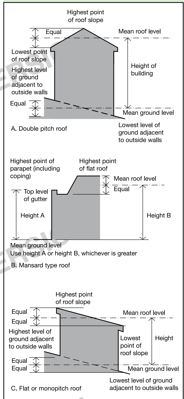
Diagram C4 Height of building
